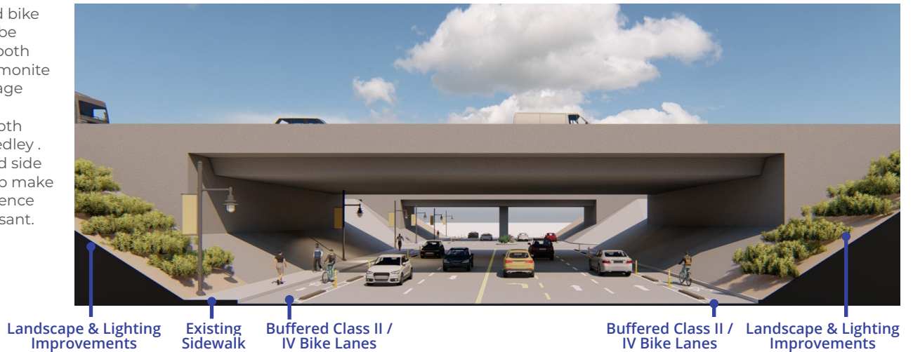
FIGURE 2.6.A | VAN BUREN UNDERPASS - CONCEPTUAL IMPROVEMENTS - BIKE PRIORITY
