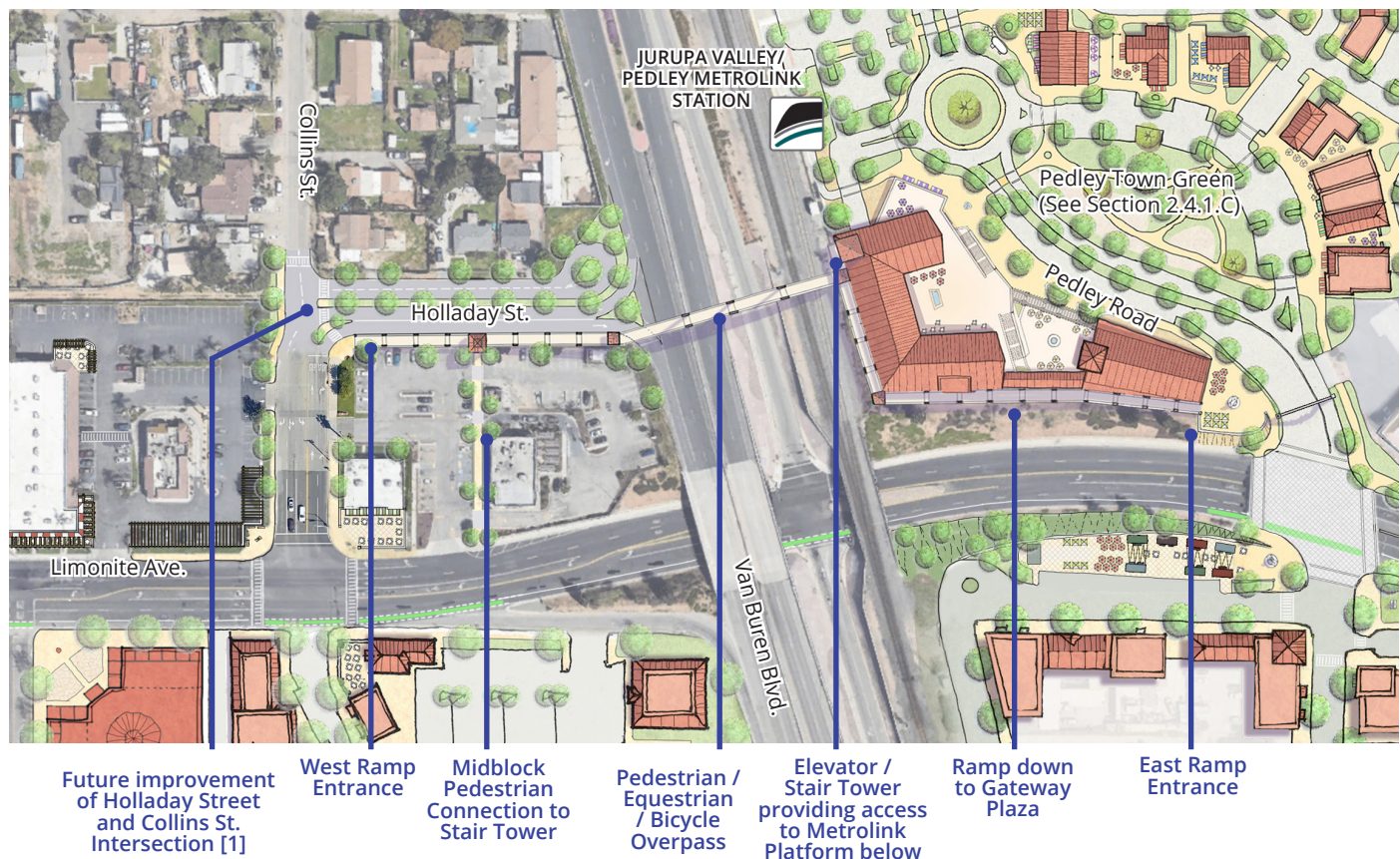
FIGURE 2.5 | CONCEPTUAL VAN BUREN CARLESS OVERPASS
